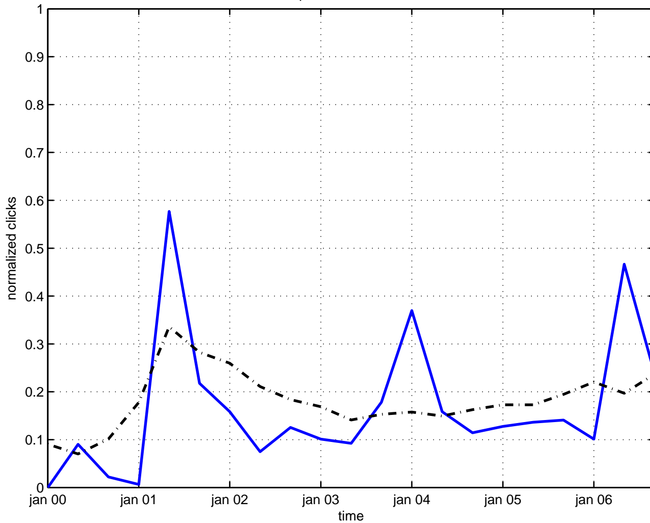
expansion heat kernel
