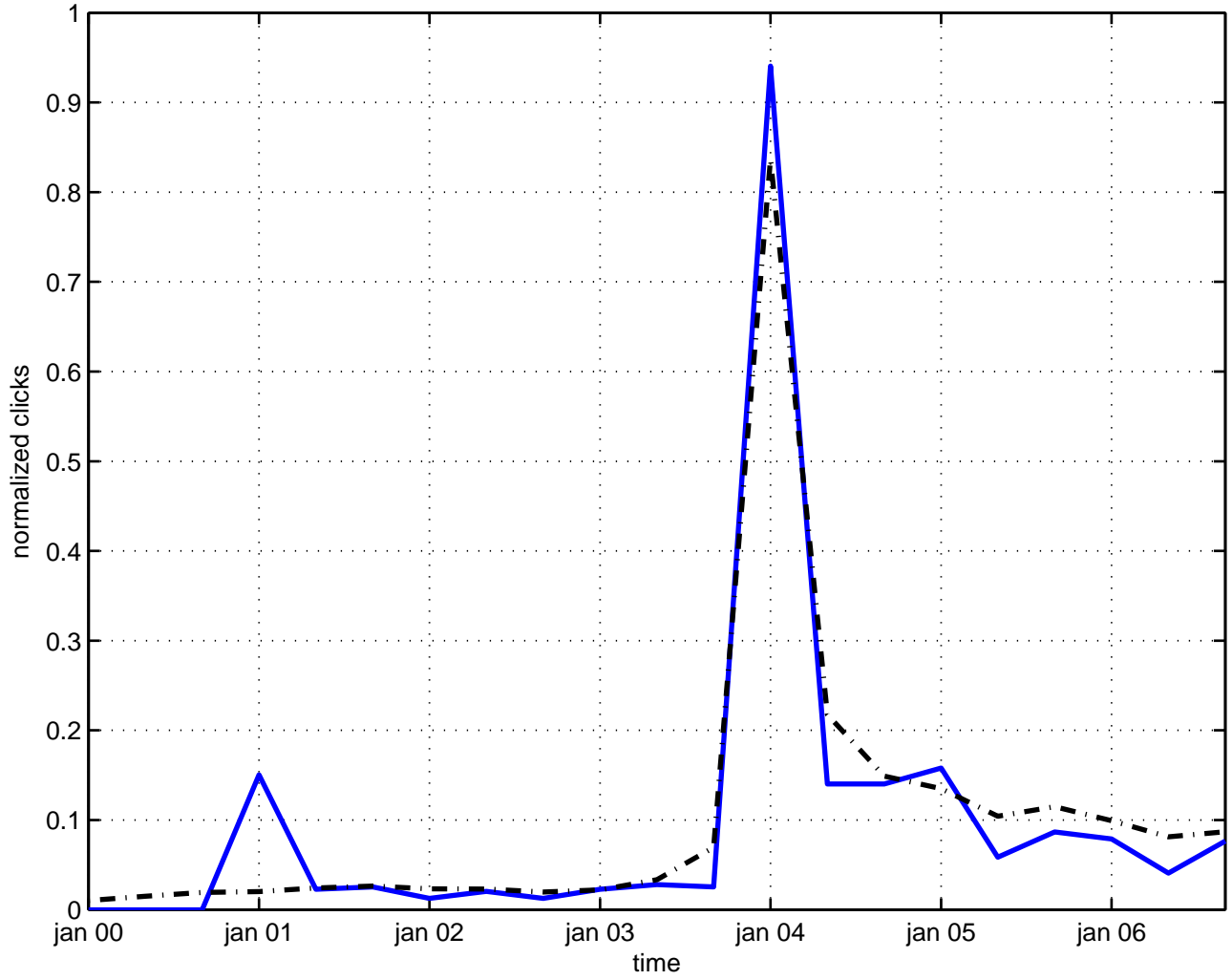
exotic statistics
