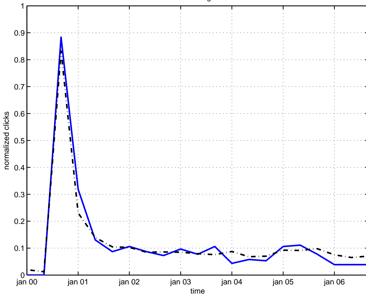
excited state graviton
