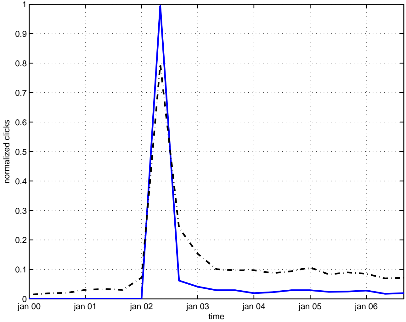
excited state atom
