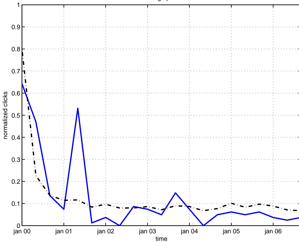
exchange photon
