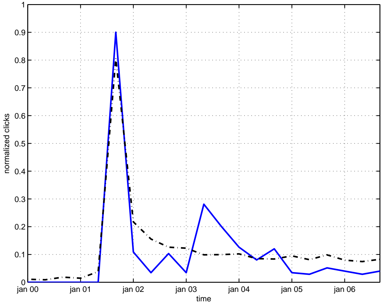
exchange particle
