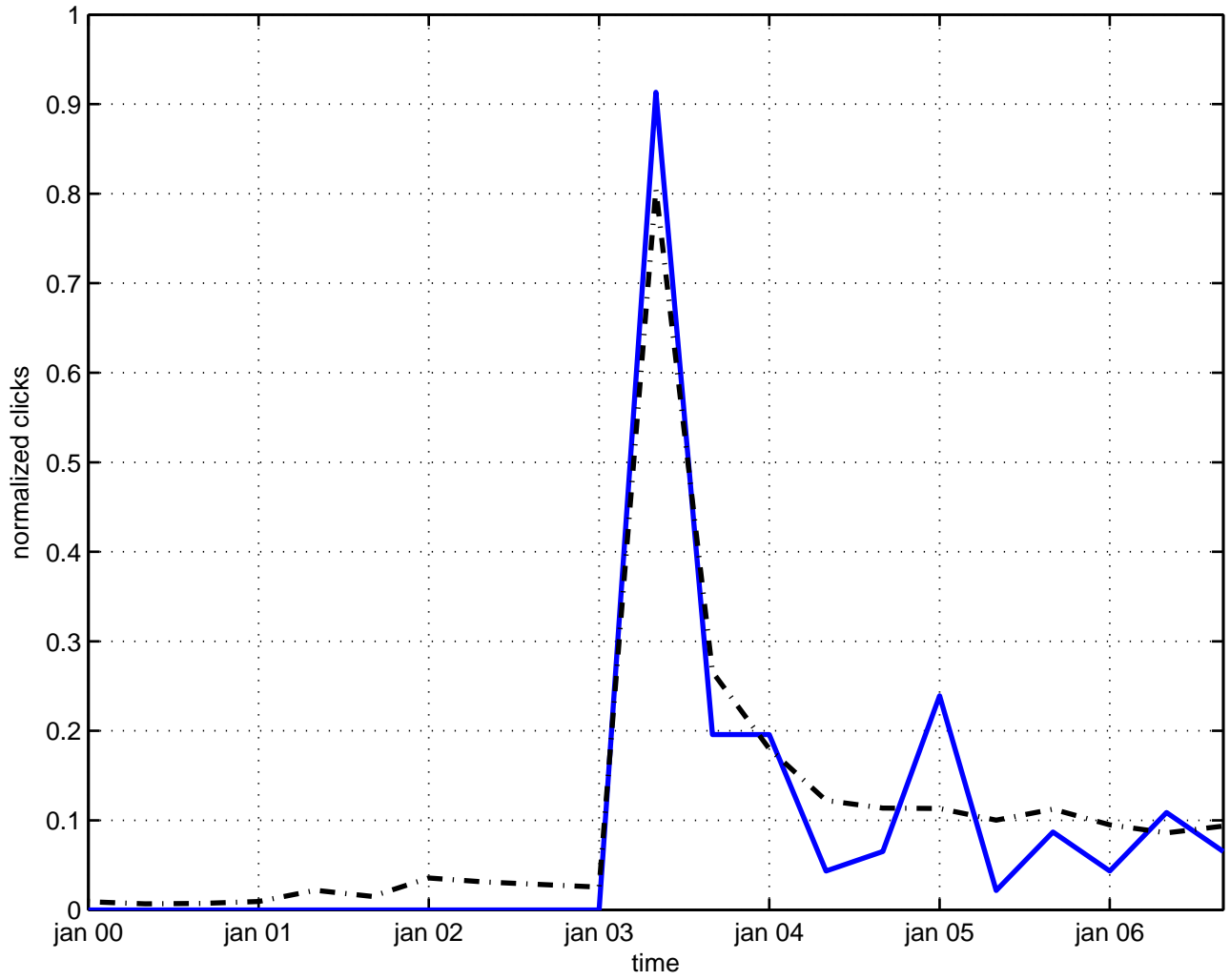
exchange group theory
