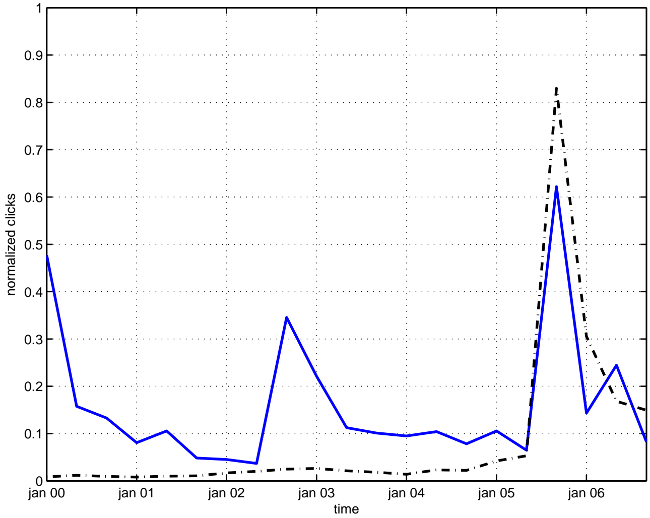
exchange graviton
