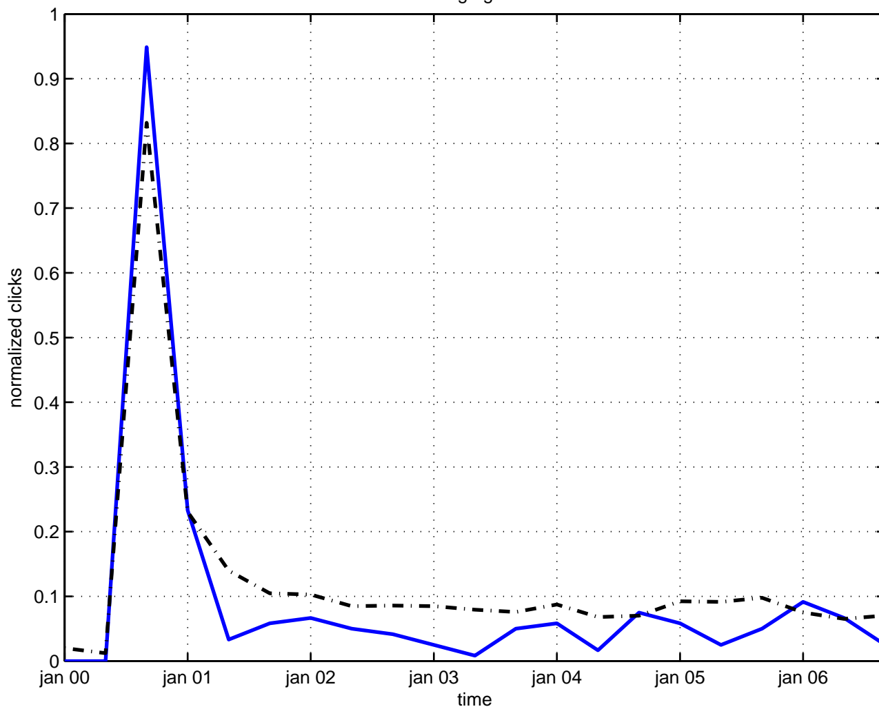
exchange gravitino
