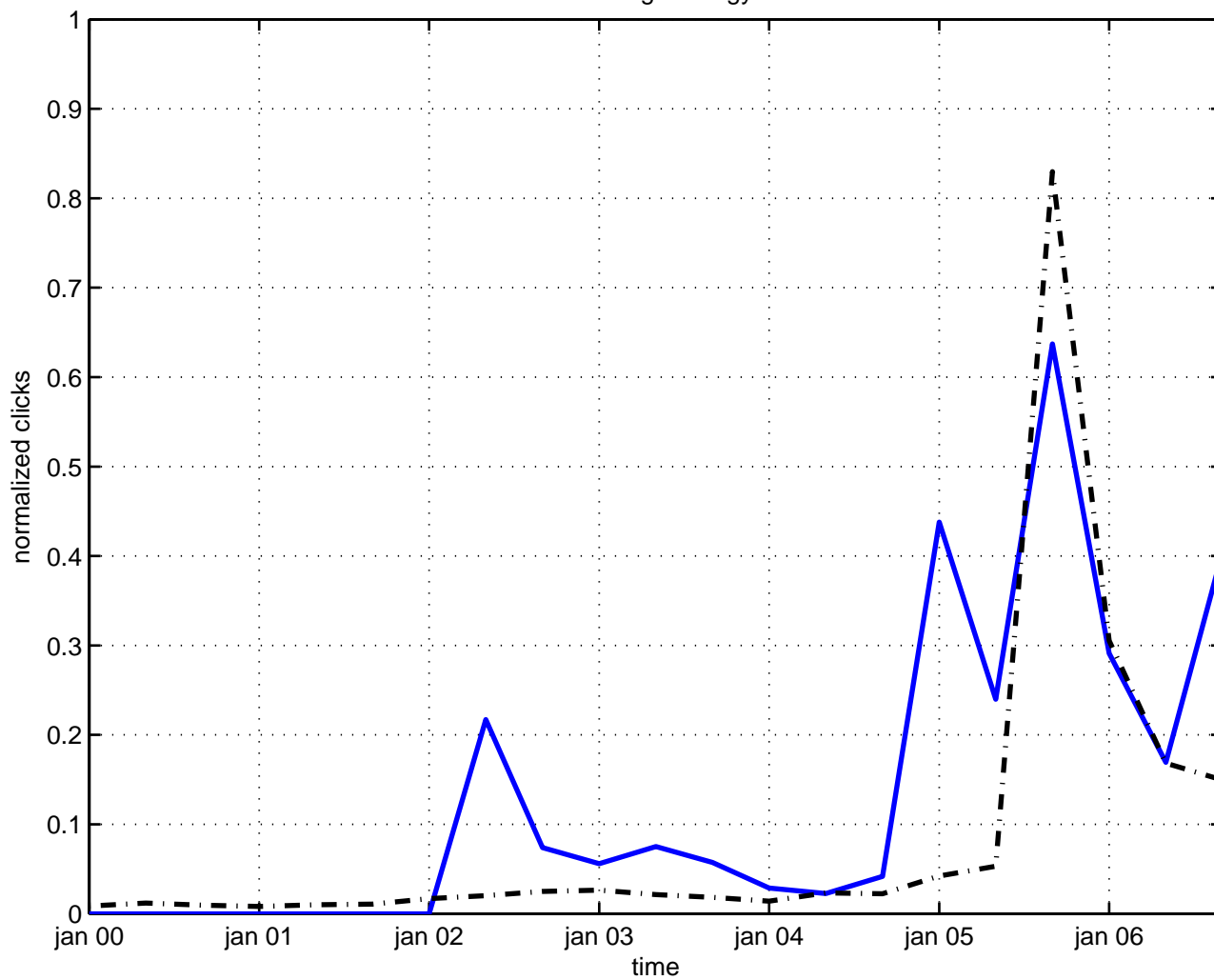
exchange energy
