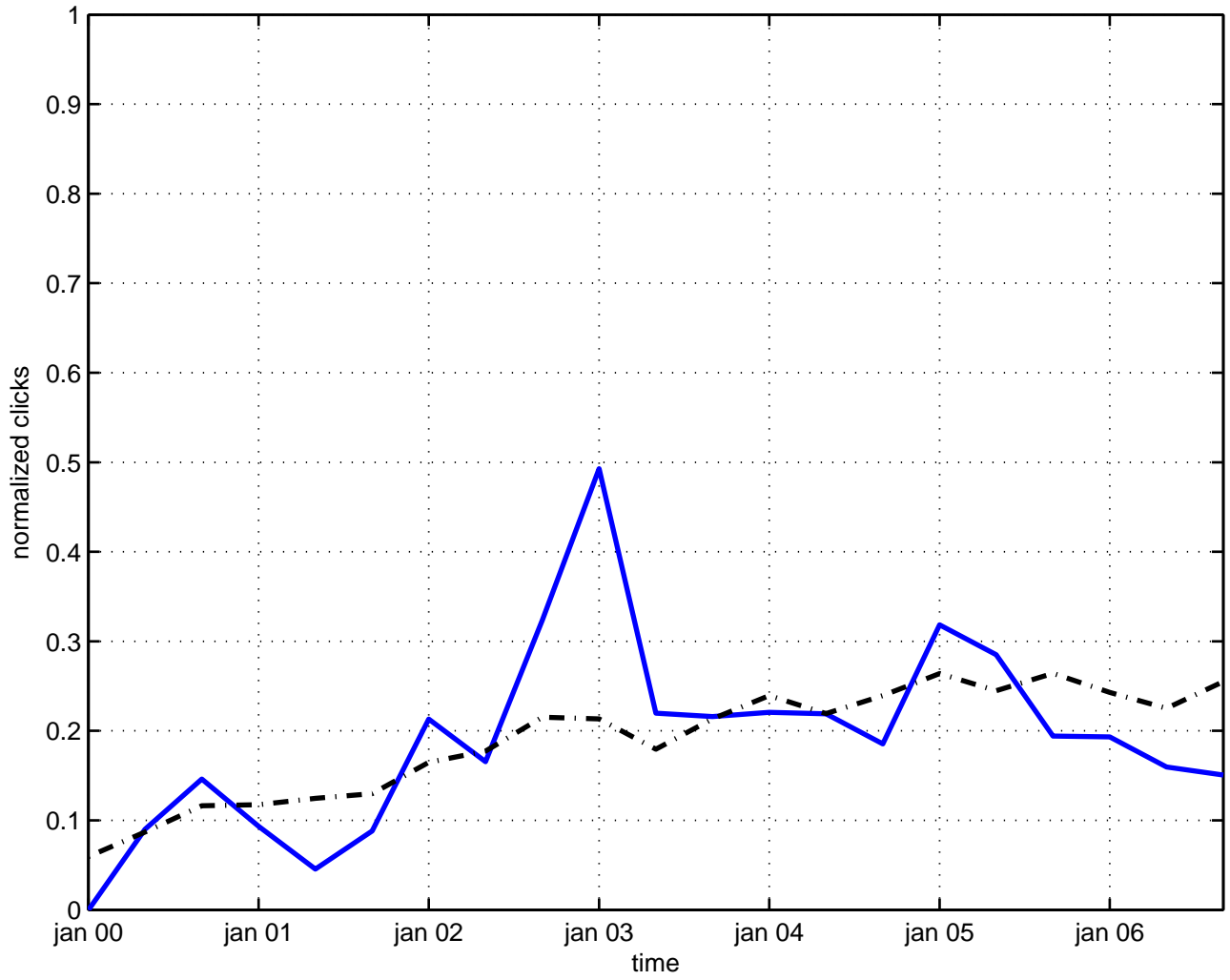
exceptional group theory
