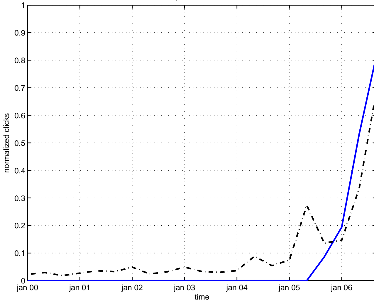
evaporation black hole
