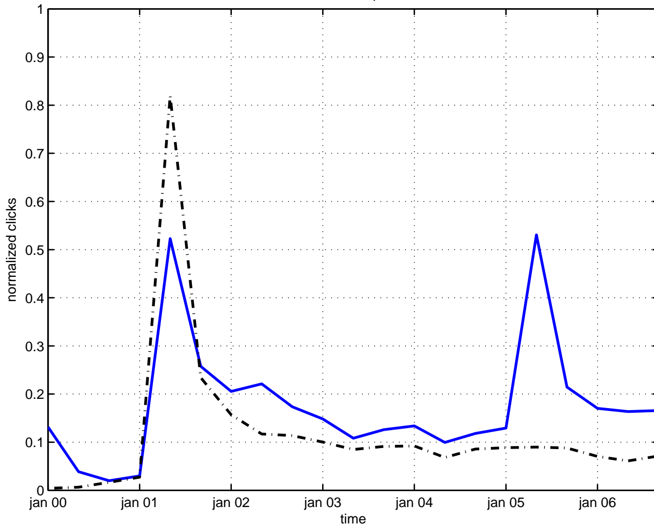
euclidean space
