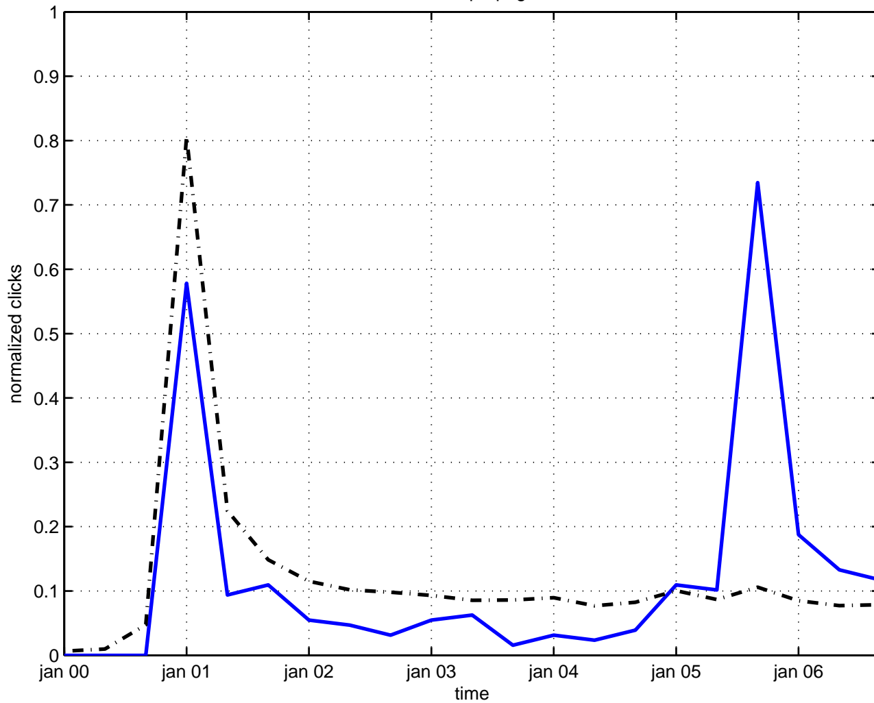
euclidean propagator
