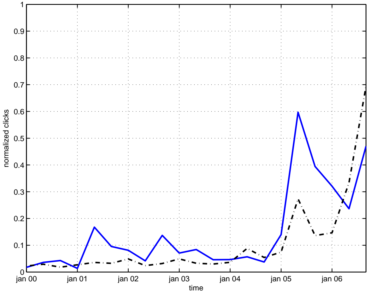
euclidean path integral
