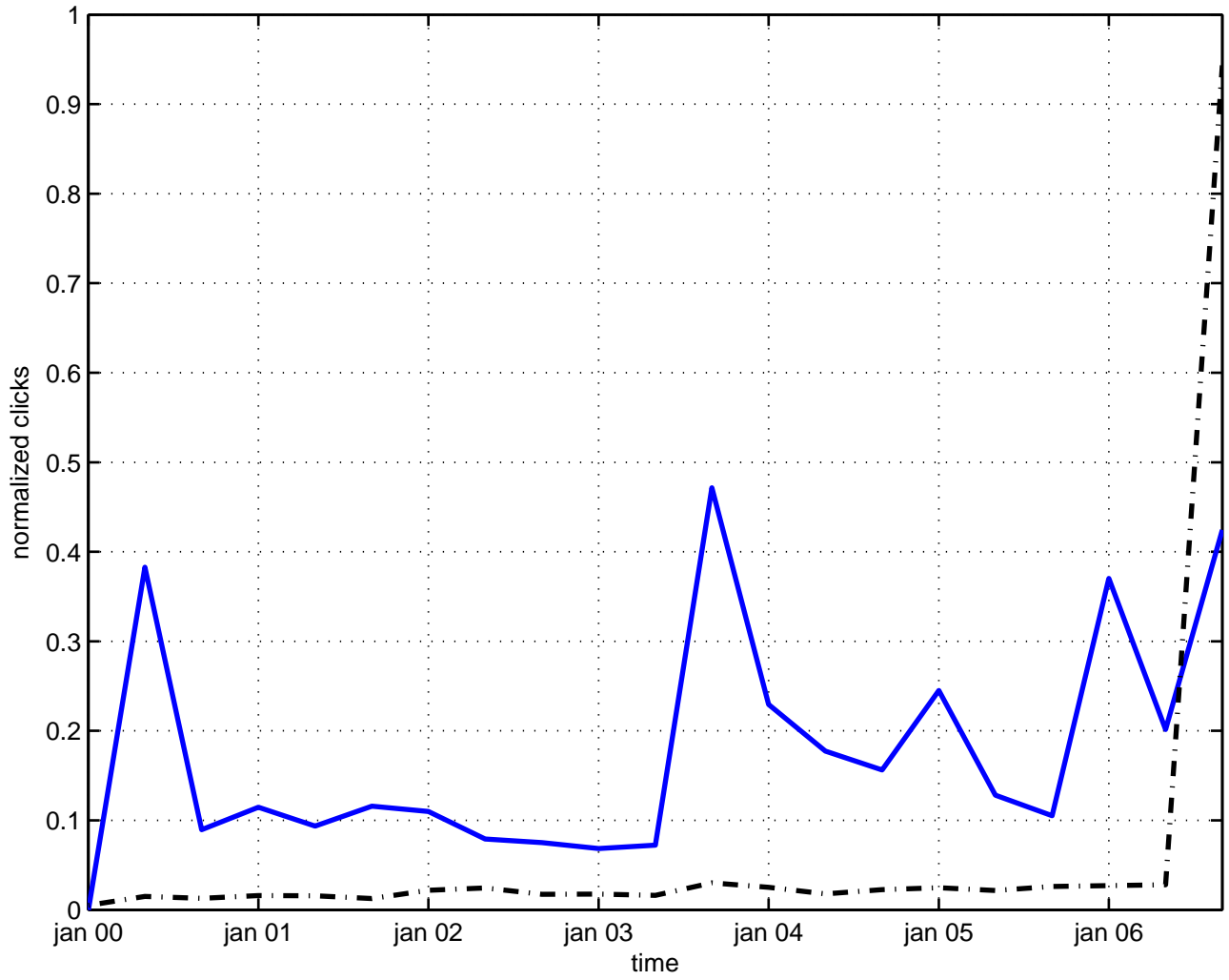
euclidean black hole
