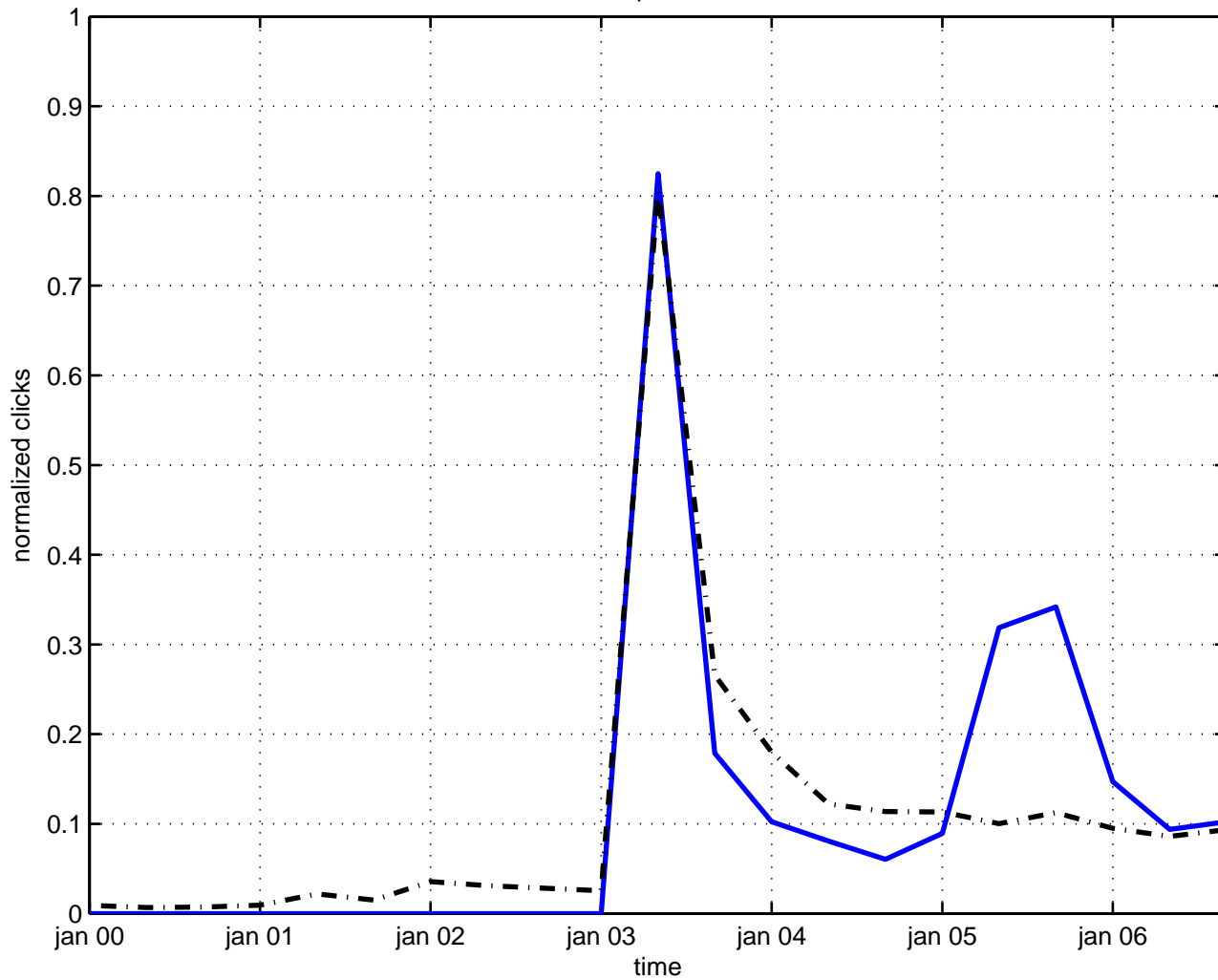
ernst space-time
