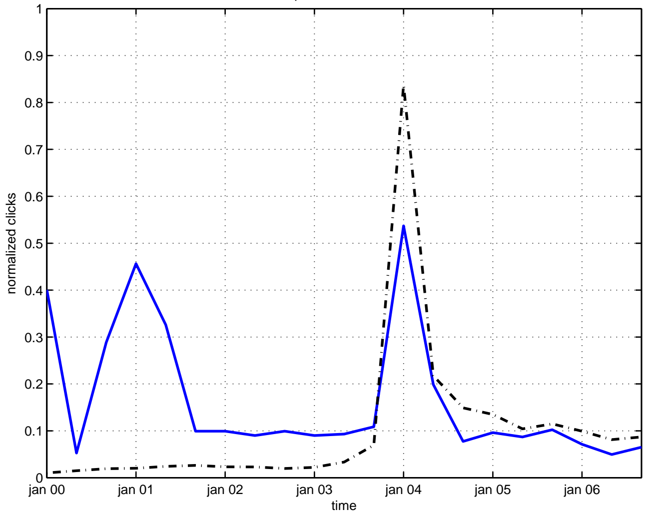
equivalence theorem
