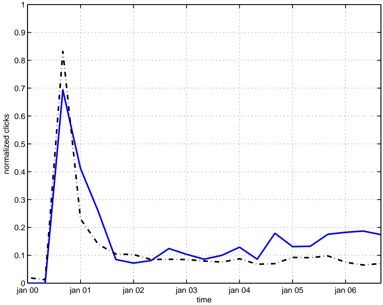
equivalence principle relativity theory
