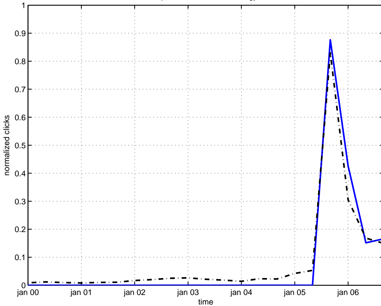
equation of state dark energy
