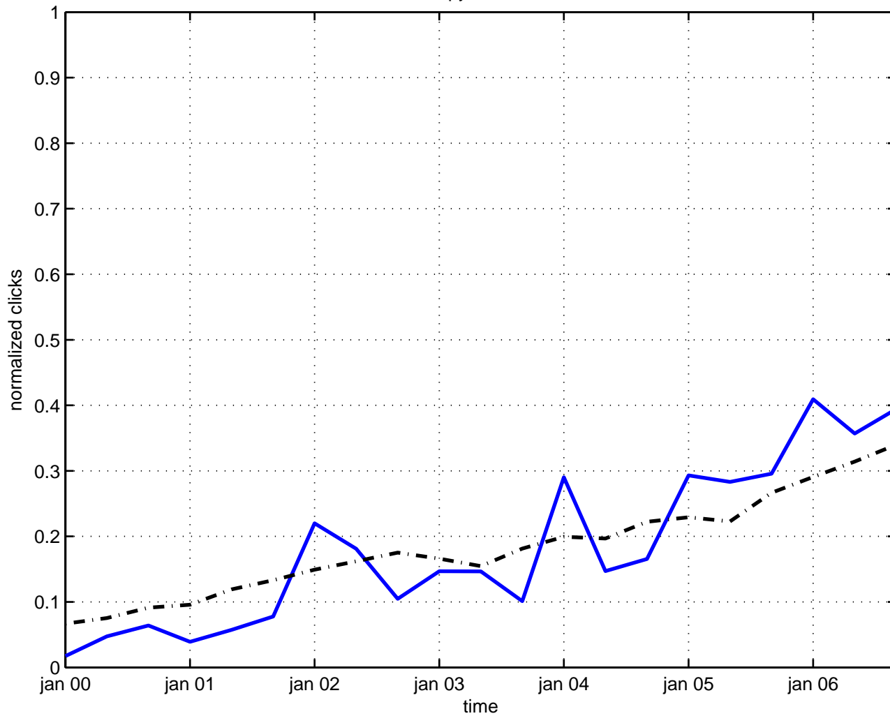
entropy black hole
