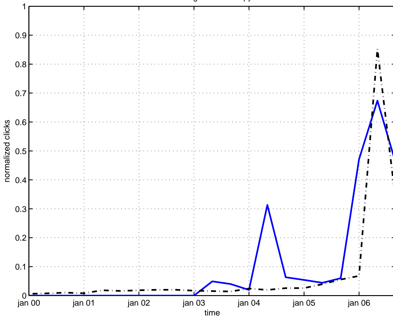
entanglement entropy
