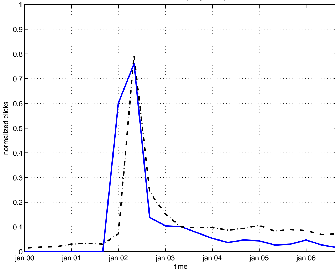
enhancement supersymmetry
