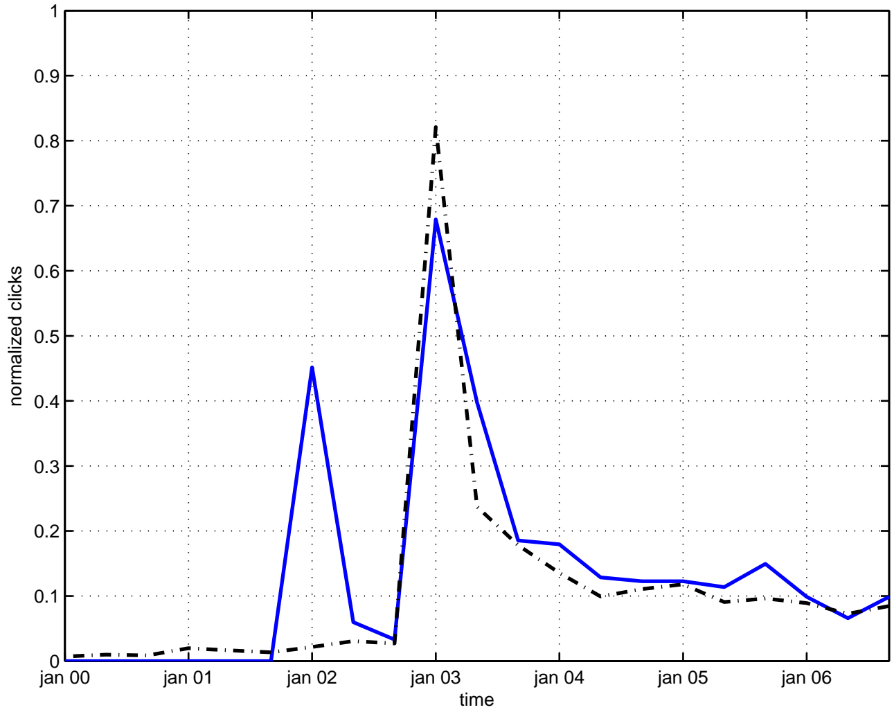
energy-momentum conservation law
