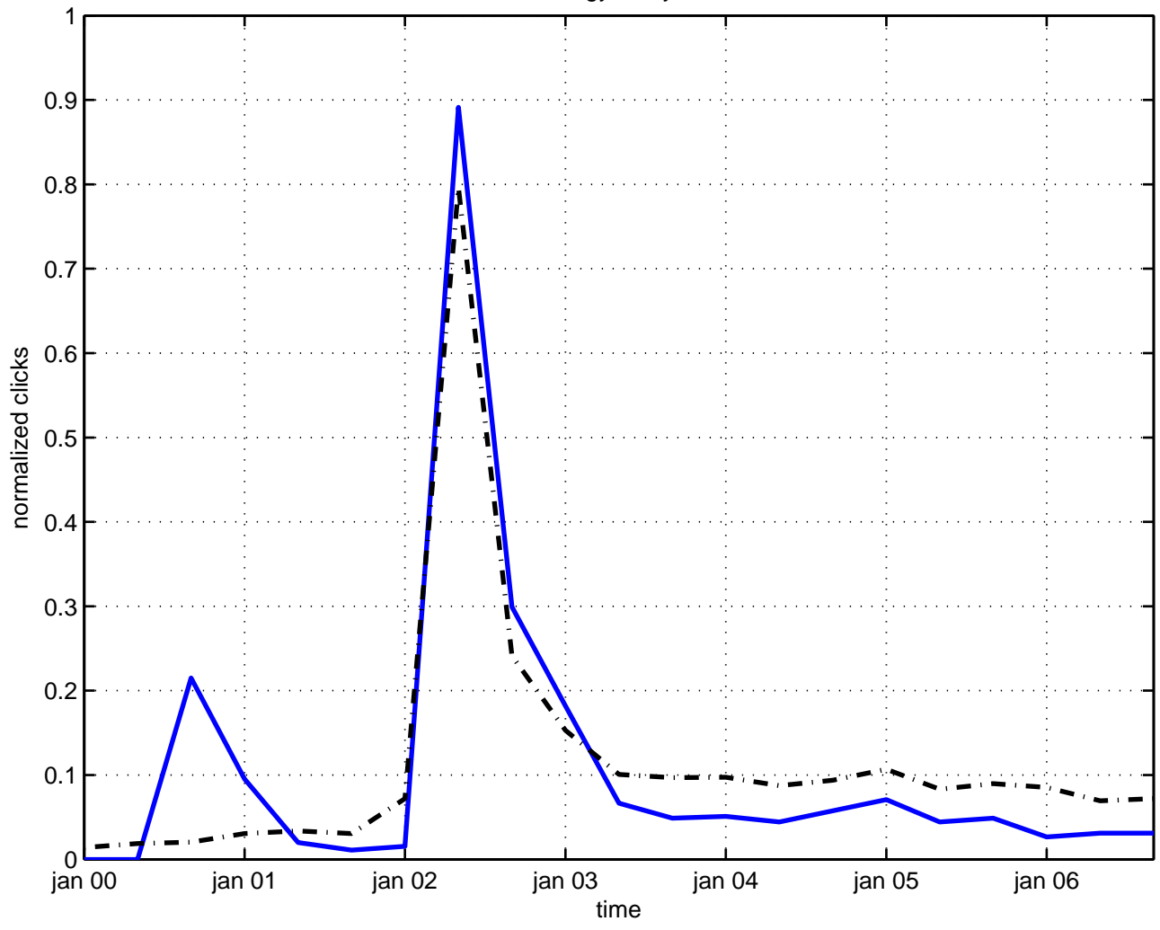
energy tachyon
