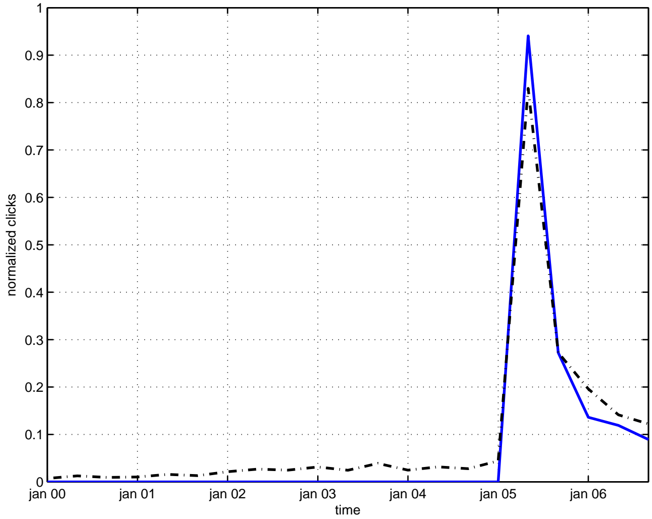
energy spectrum n
