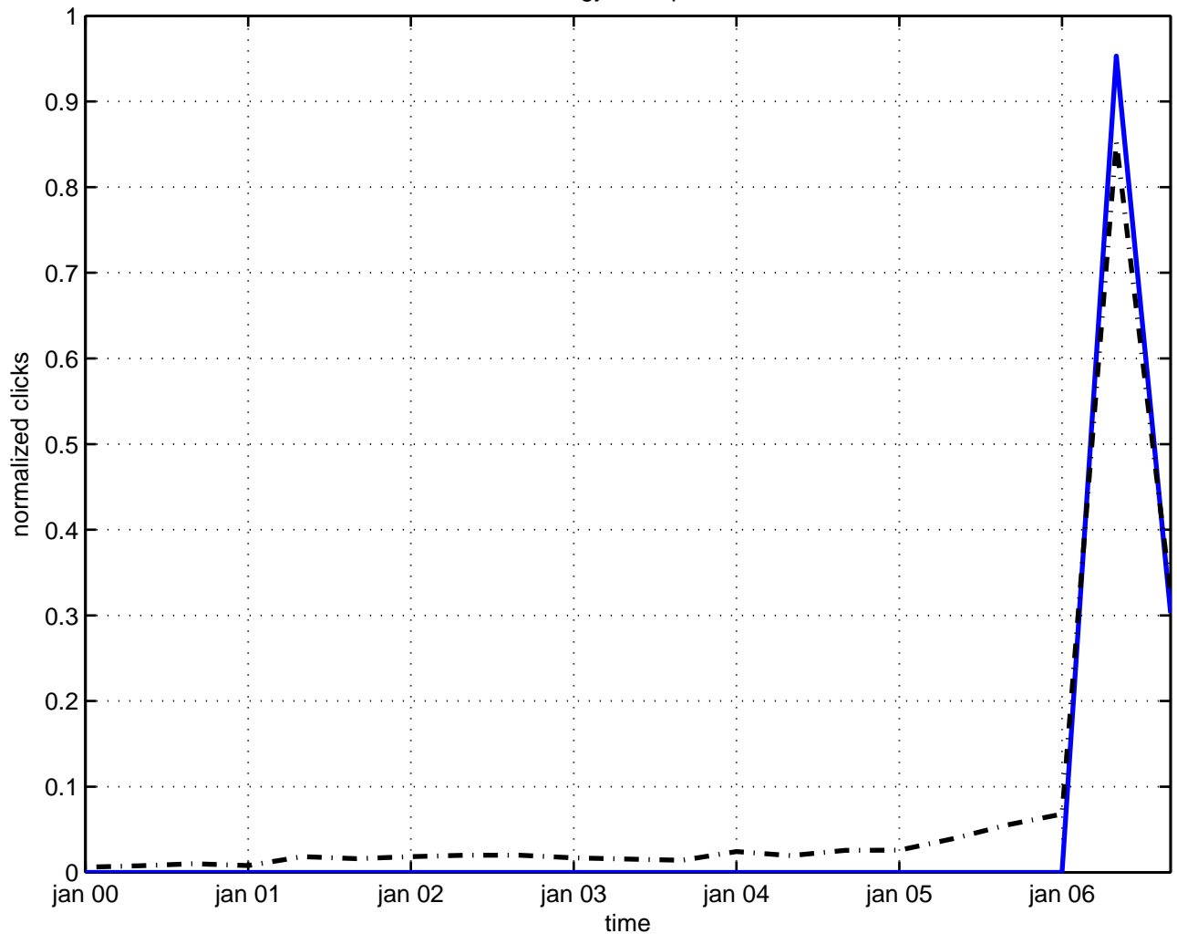
energy loss quark
