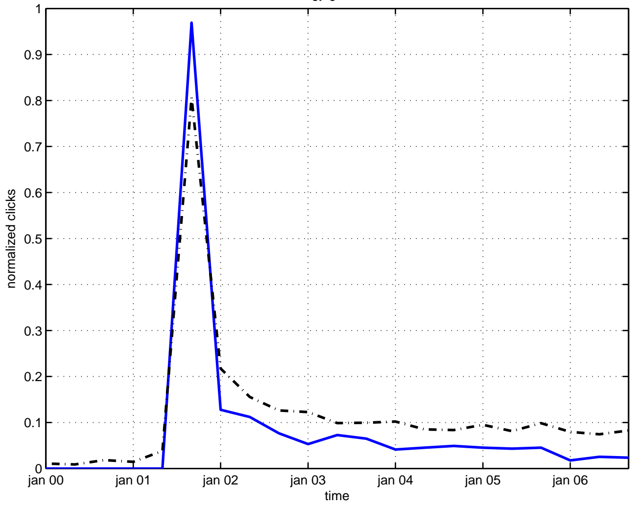
energy gravitation
