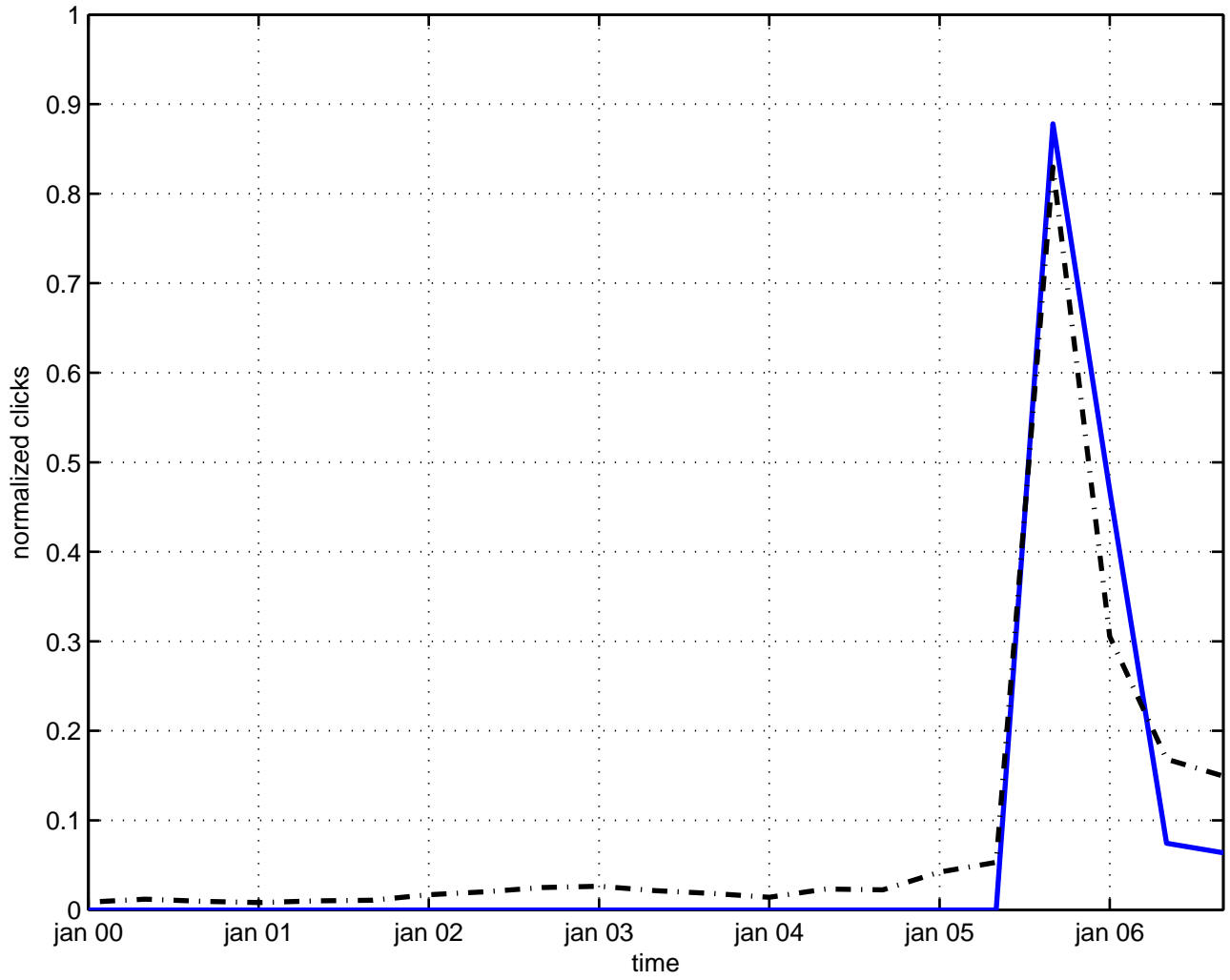
energy electron
