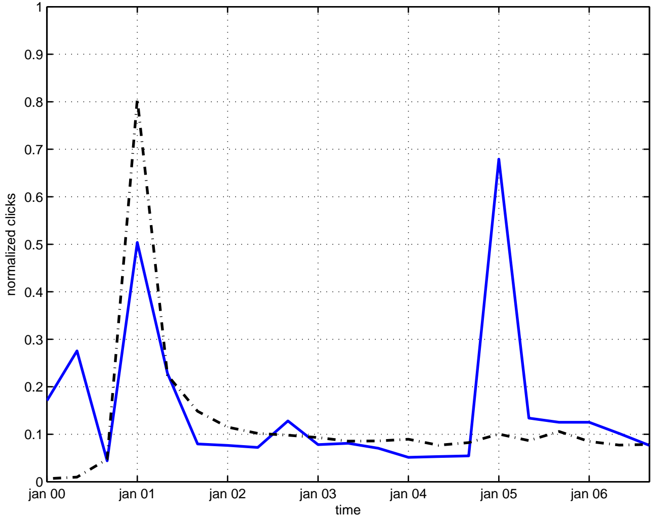
energy bound state
