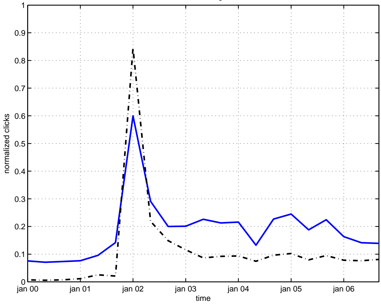
embedding
