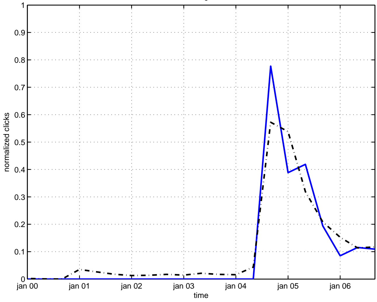
embedding tensor
