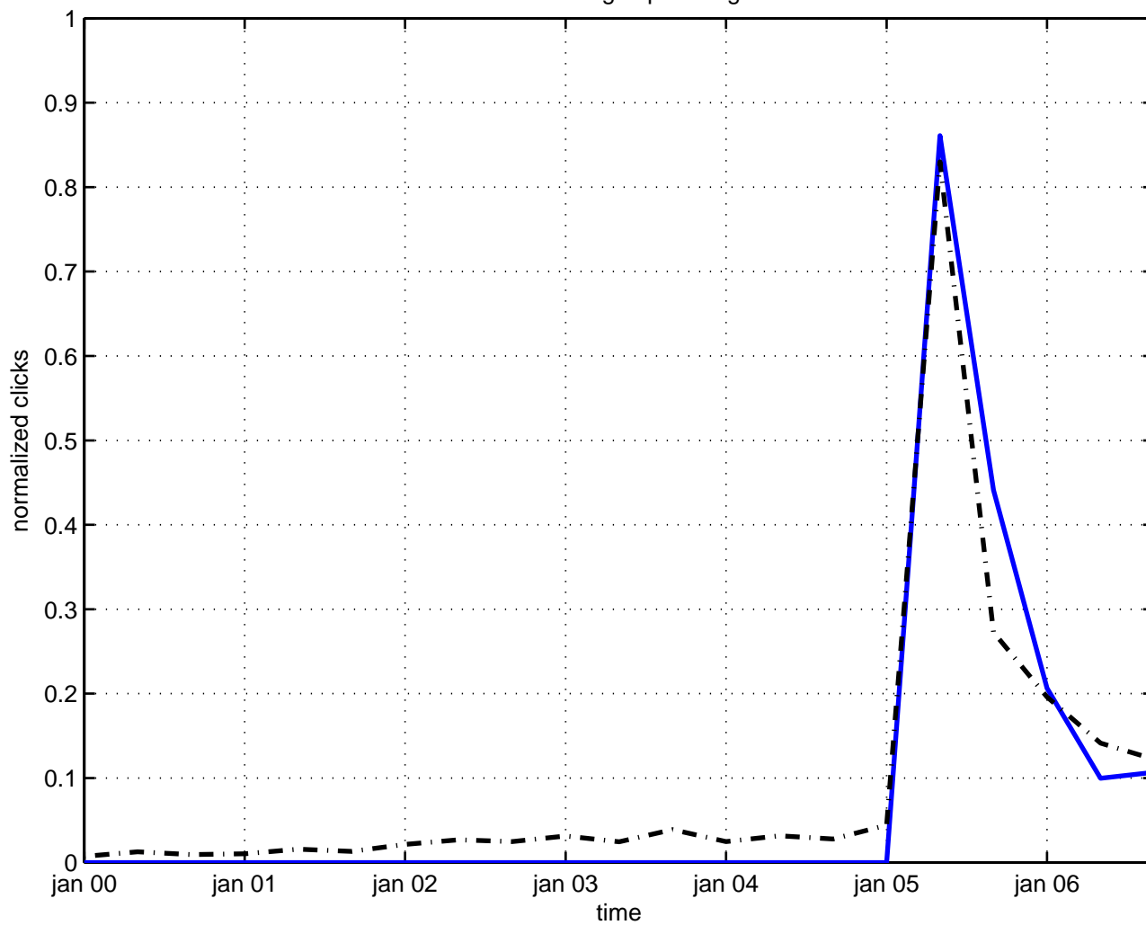
embedding superstring
