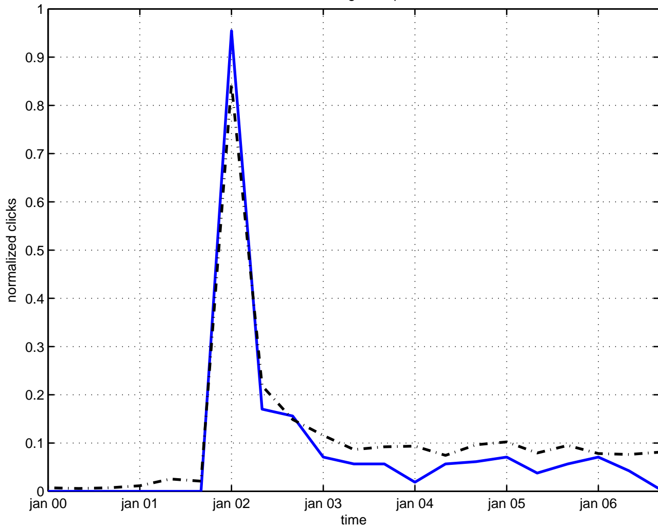
embedding monopole
