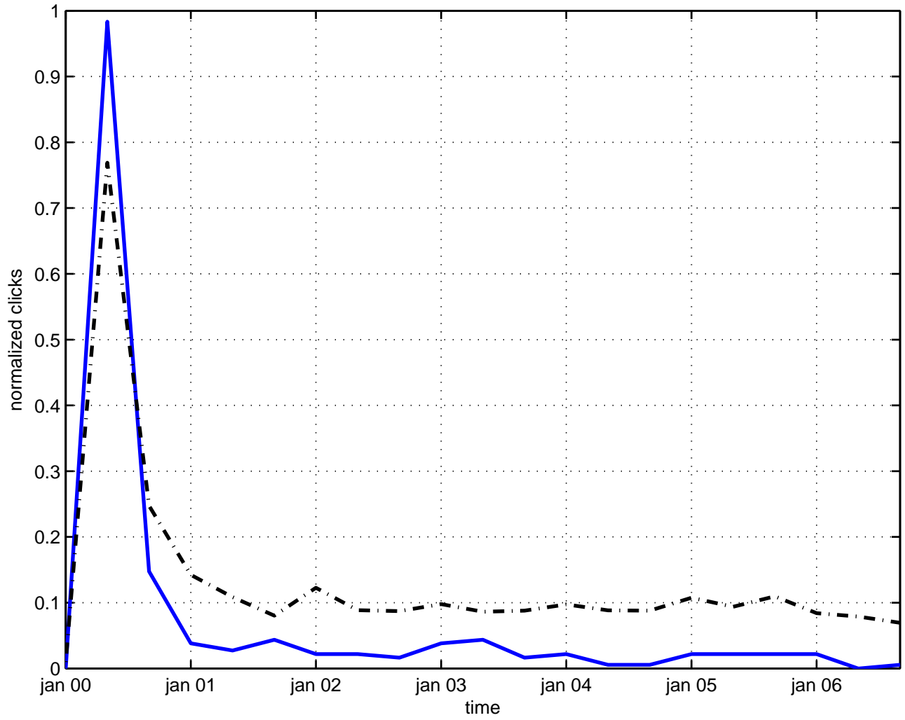
embedding m-theory
