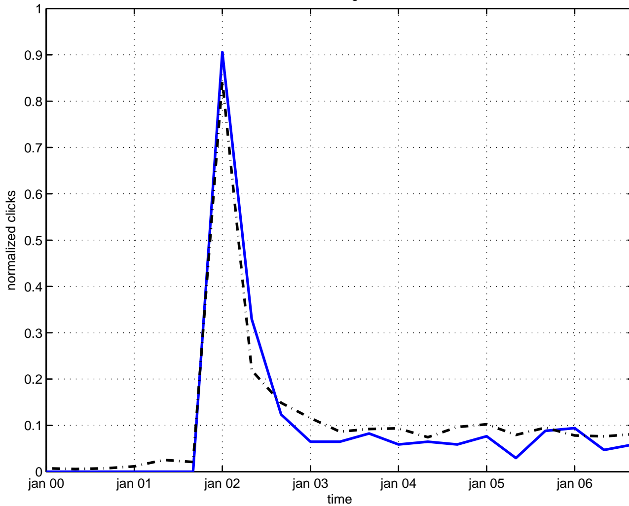
embedding kink
