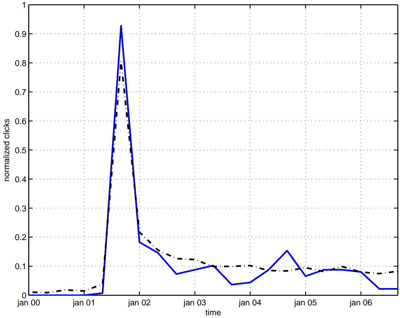
embedding group theory
