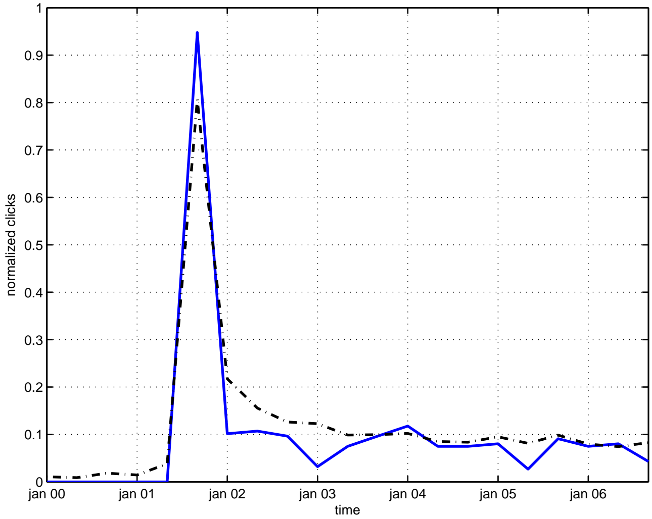
embedding friedman model
