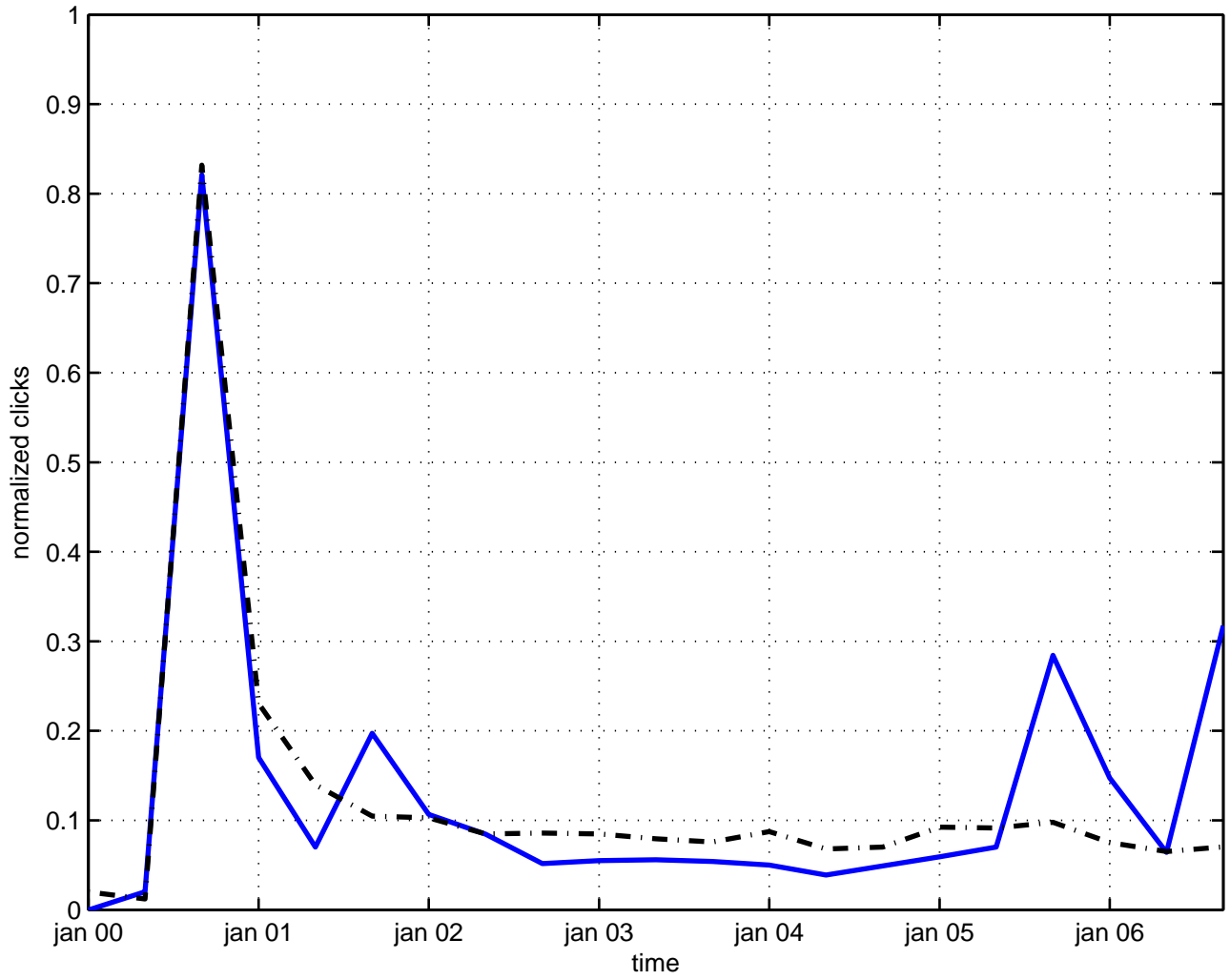
electron
