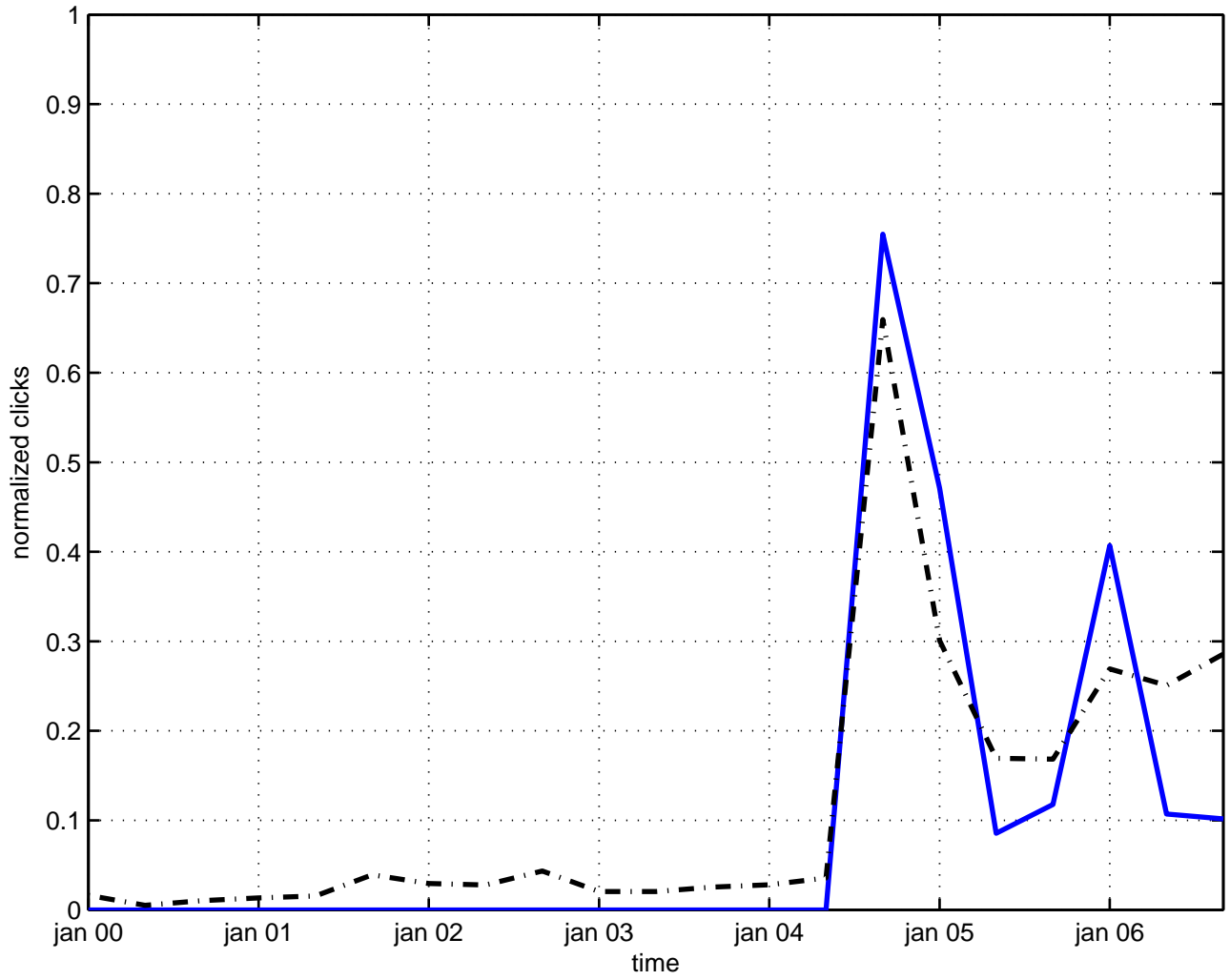
electromagnetic fluctuation
