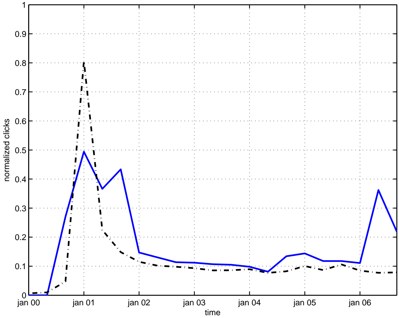
electromagnetic duality
