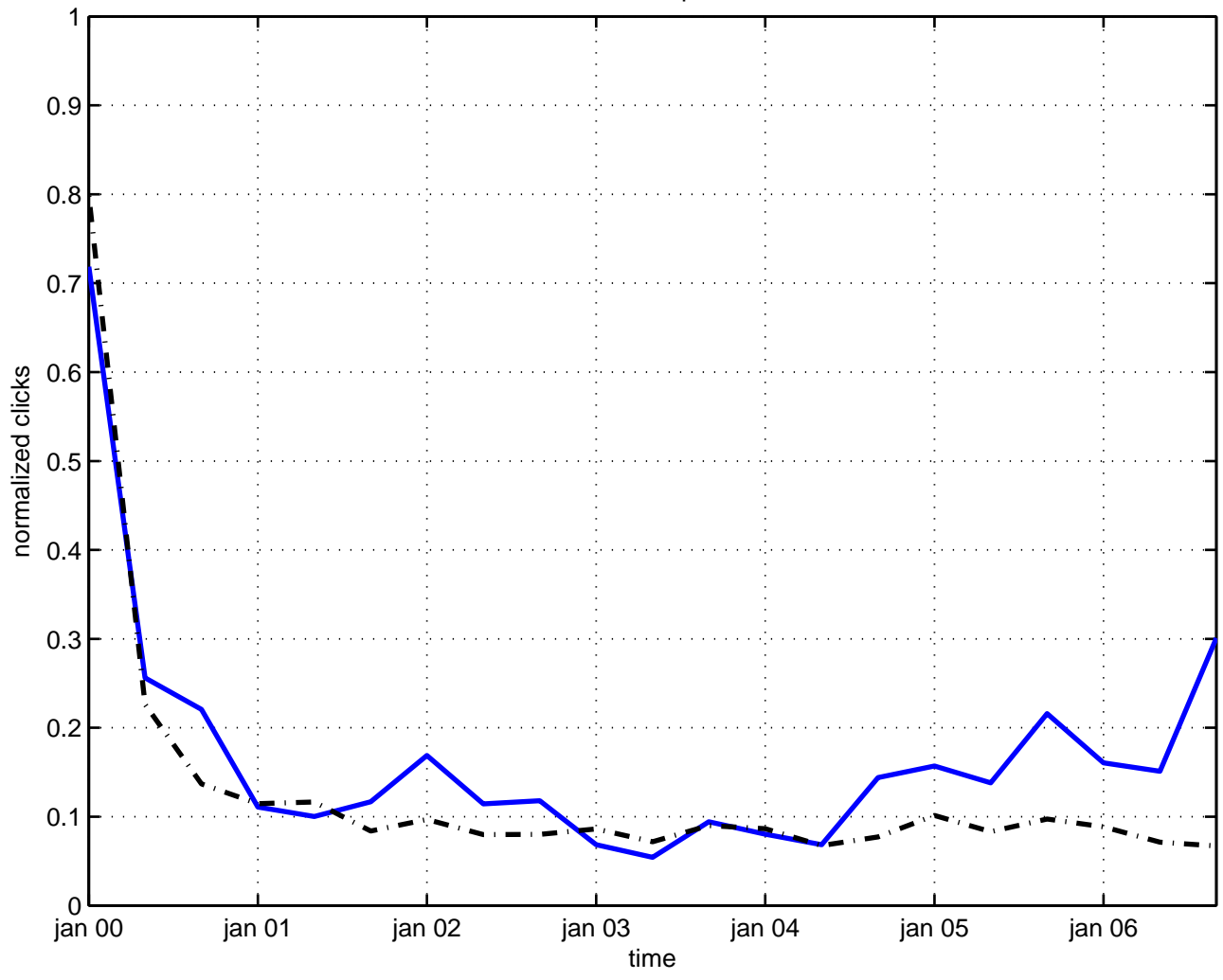
electric dipole
