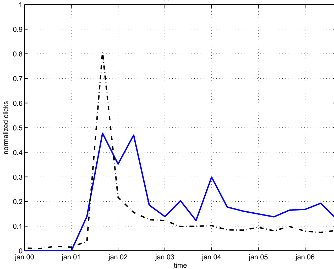
ekpyrotic model
