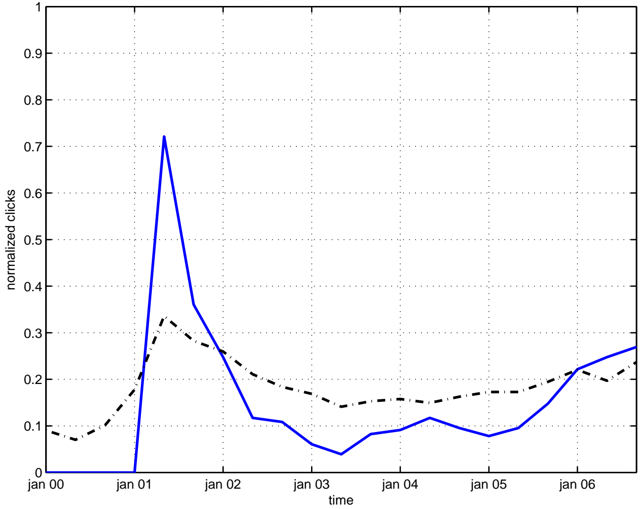
effective potential radion
