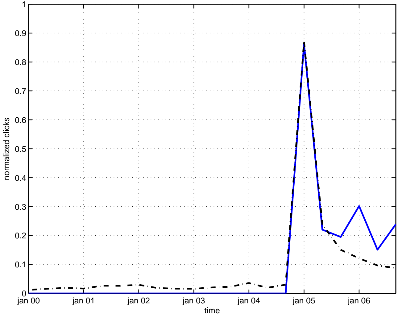
effective potential inflaton
