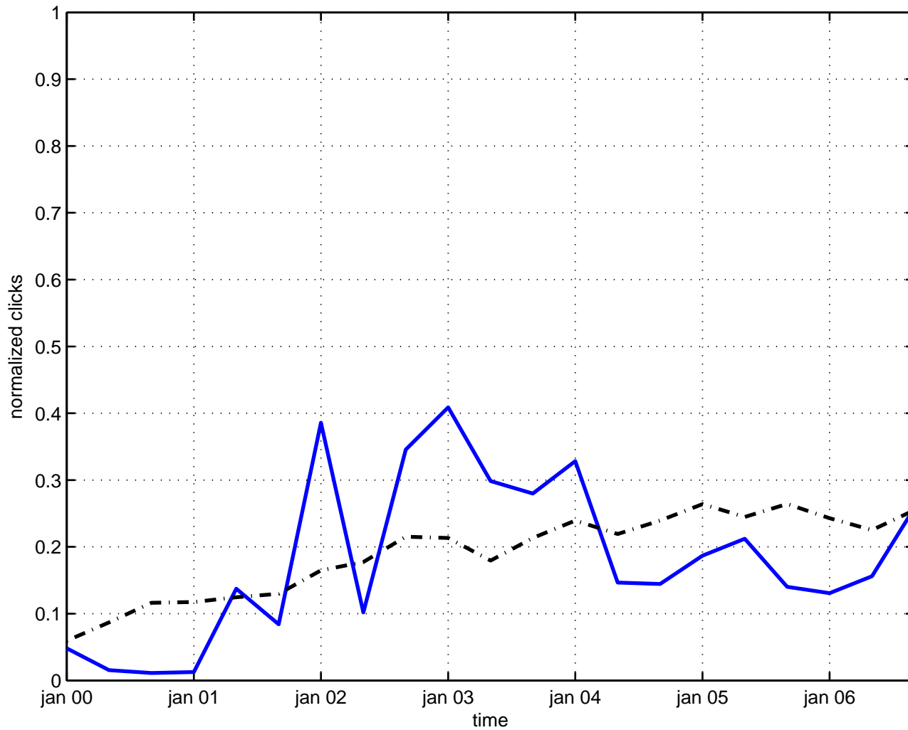
effective hamiltonian
