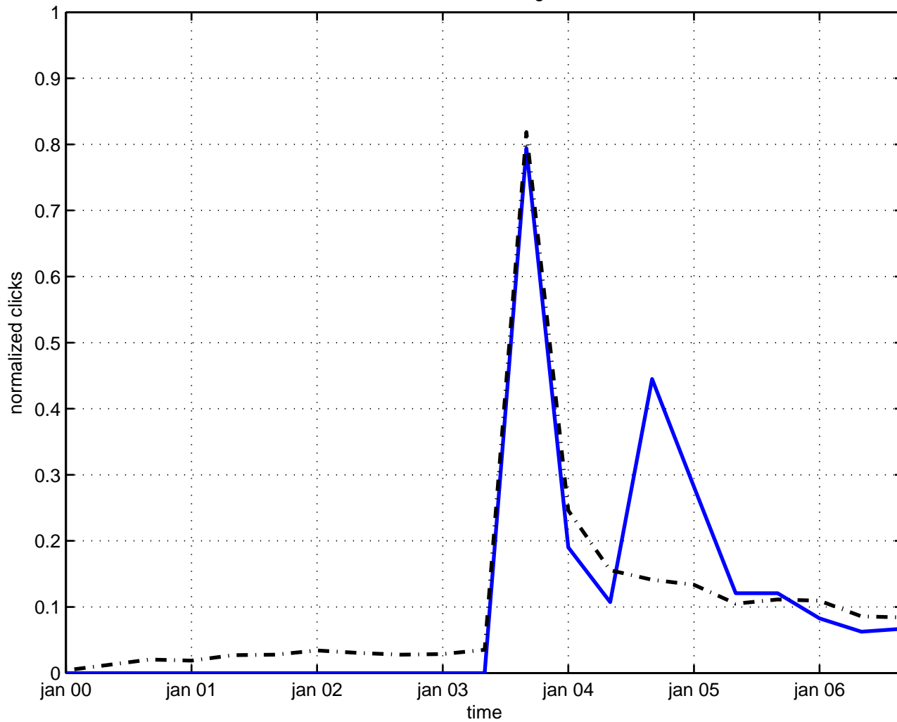
effective action string model
