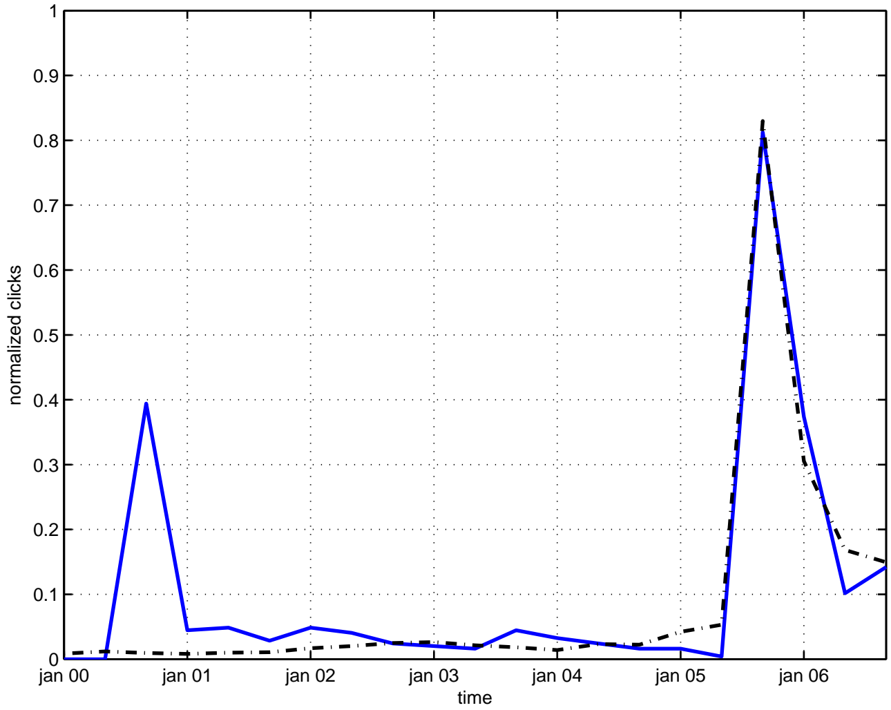
effective action quantum chromodynamics
