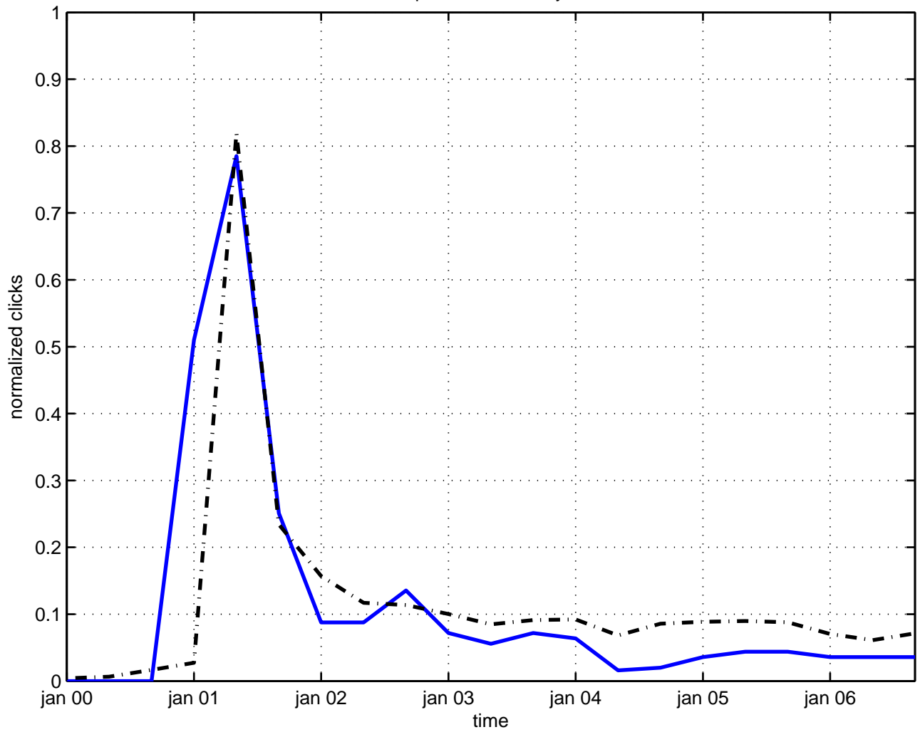
effect quantum electrodynamics
