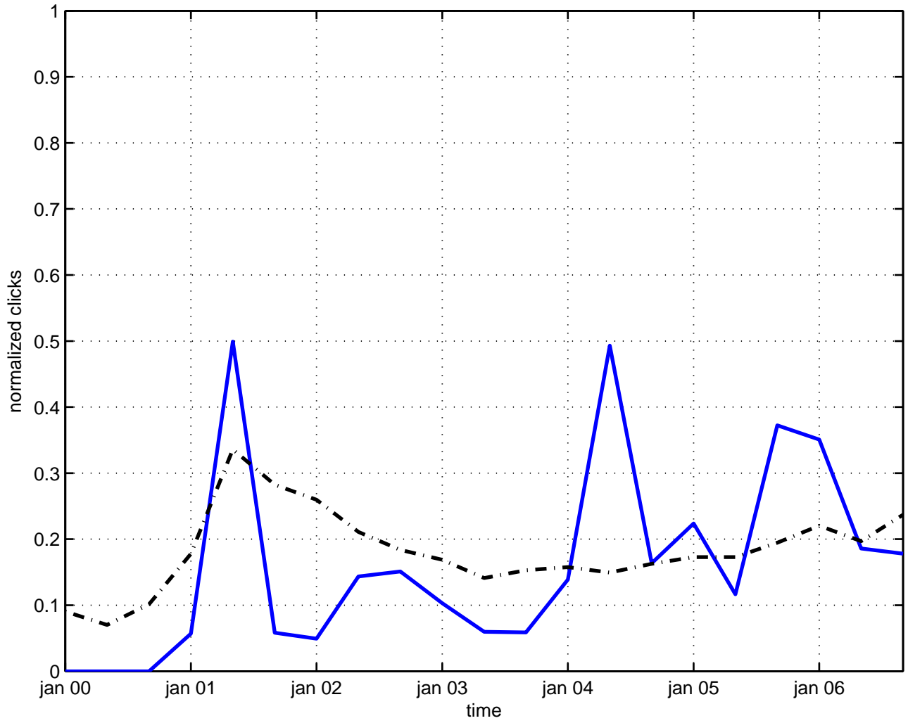
effect gravitation
